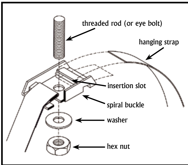
Spiral Buckle with threaded rod
