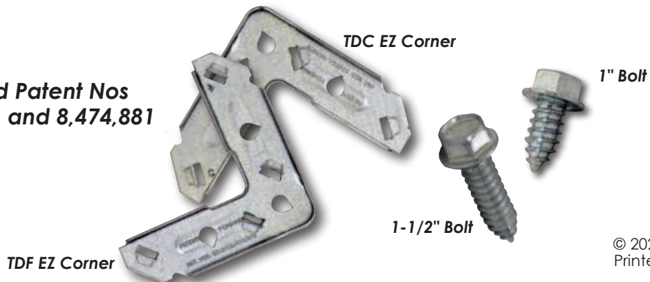
Self-piloting screw tip of the bolt self-aligns the corners and ductwork, eliminating the need for an alignment tool and clamping. 1-1/2" bolt shown.
