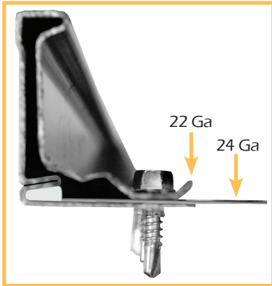
Stainless Steel High Head Pro Point screws piercing through 22 gauge flange and 24 gauge ductwork.
